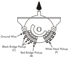
"Ground Side" Wafer Layout
