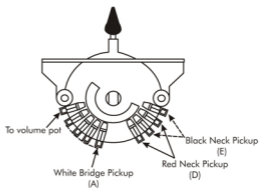
"Hot Side" Wafer Layout
