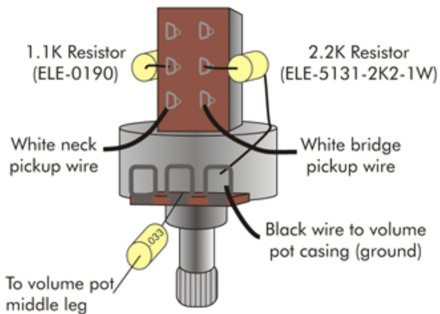
Push-pull tone pot:
