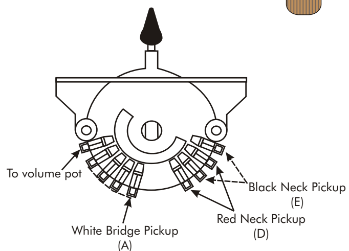
"Hot Side" Wafer Layout
