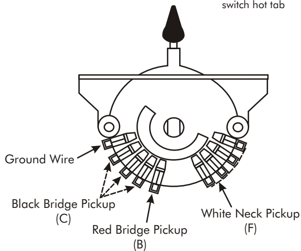
"Ground Side" Wafer Layout
