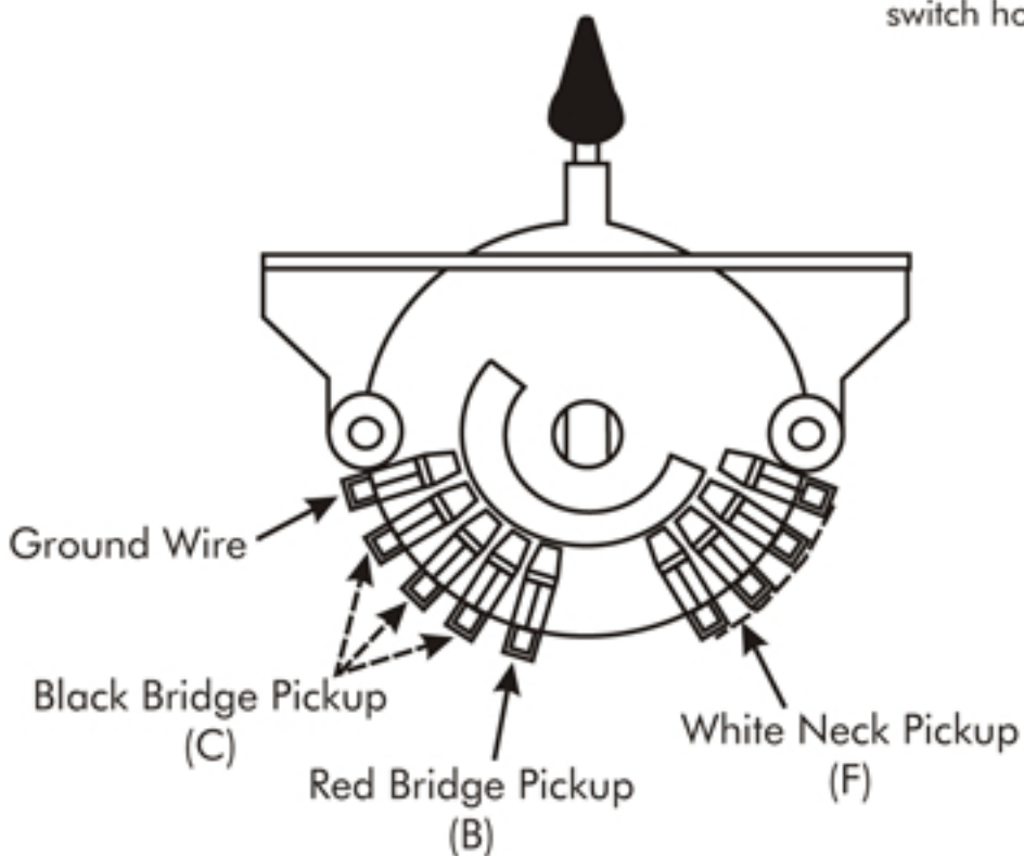
"Ground Side" Wafer Layout
