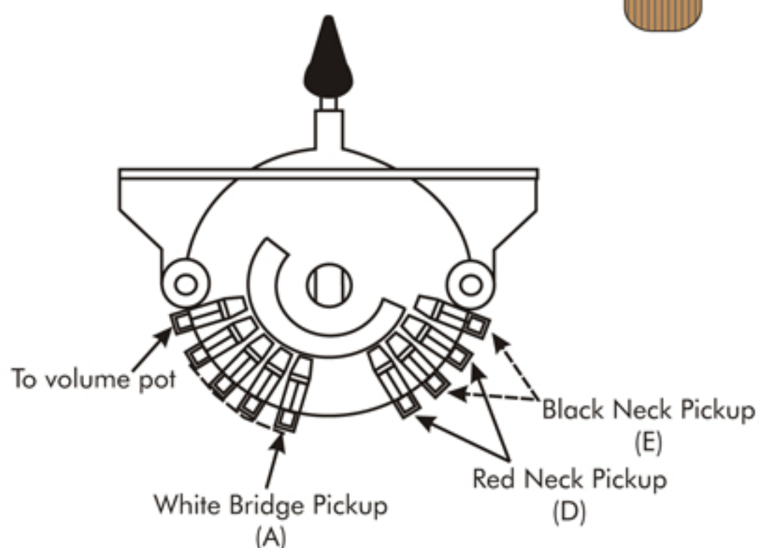
"Hot Side" Wafer Layout
